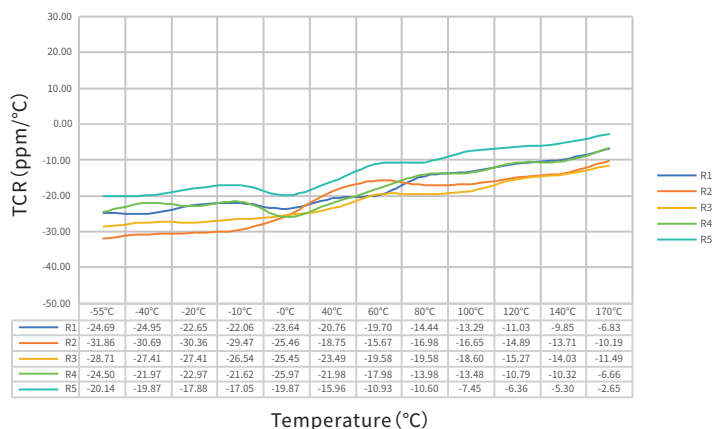
TCR Test Curve - SEWF3951 0.4mΩ
