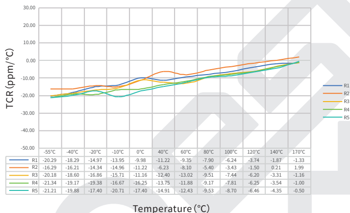
TCR Test Curve - SEWF3951 0.4mΩ
