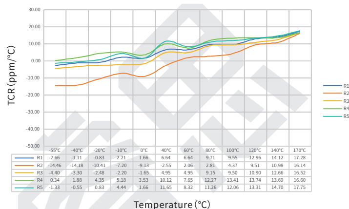
TCR Test Curve - SEWF3951 0.8mΩ
