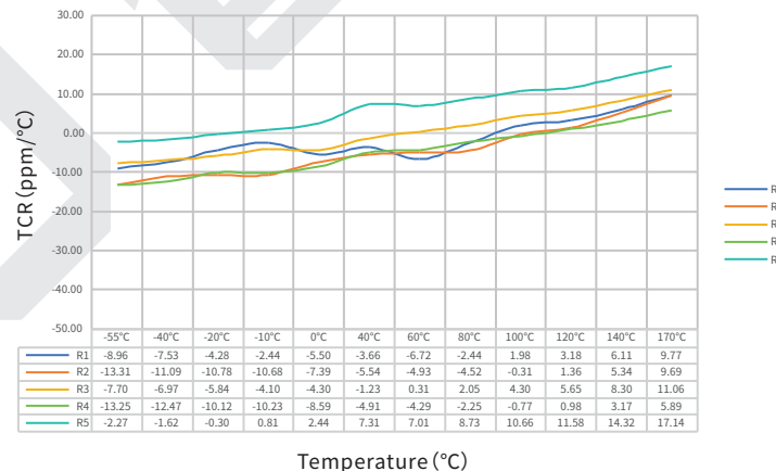
TCR Test Curve - SEWF3951 0.8mΩ
