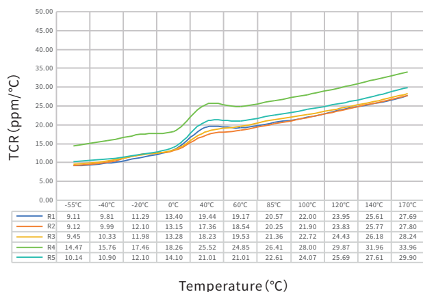
TCR Test Curve - PEWF2512 2mΩ
