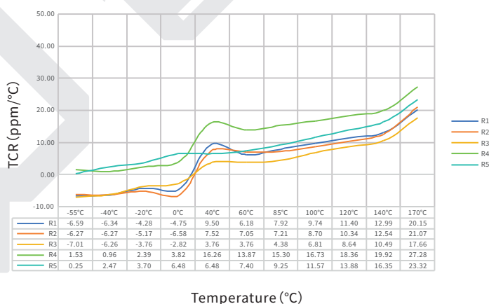
TCR Test Curve - PEWF2512 5mΩ
