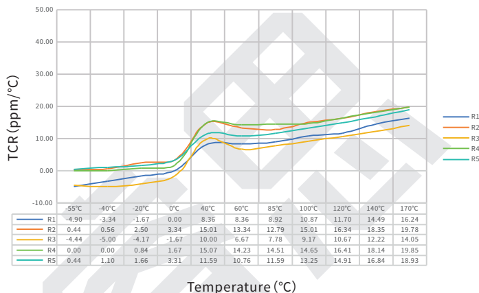
TCR Test Curve - PEWF2512 3mΩ
