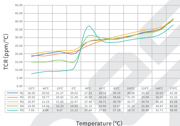
TCR Test Curve - PEWF2512 4mΩ
