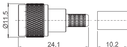
EMU-3901 MINI UHF MALES STRAIGHT CRIMP FOR CABLE - RG 58/U - RG 59/U - RG 6/U
