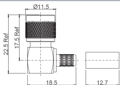
EMU-3902 MINI UHF MALE R/A FOR CABLE - RG 58/U - RG 59/U - RG 6/U
