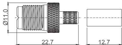
EMU-3801 MINI UHF JACK STRAIGHT CRIMP FOR CABLE - RG 58/U - RG 59/U - RG 6/U
