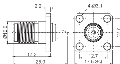
EMU-5801 MINI UHF JACK FOR SOLDERING WITH SQUARE FLANGE
