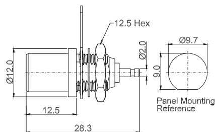
EP-5802 PAL JACK BULKHEAD FRONT PANEL MOUNT
