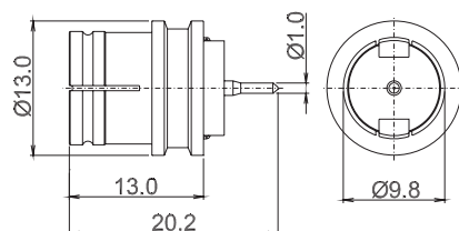
EP-5803 PAL JACK STRAIGHT PANEL MOUNT
