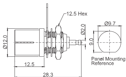
EP-5902 PAL MALE BULKHEAD FRONT PANEL MOUNT
