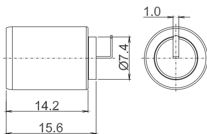
EP-5801 PAL JACK PANEL MOUNT
