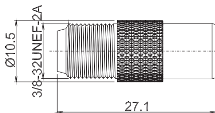
EP-6006 PAL MALE TO F JACK
