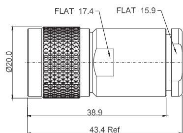
EN-2901 N MALE CLAMP STRAIGHT FOR CABLE - RG 8A/U - RG 11A/U - RG 213/U
