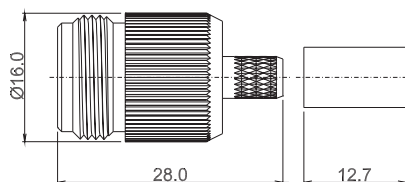
EN-3801 N JACK STRAIGHT CRIMPING FOR CABLE - RG 58/U - RG 59/U - RG 6/U
