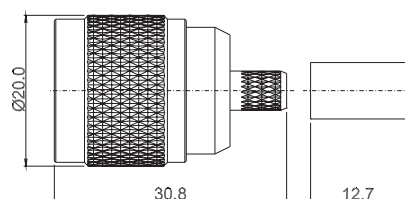
EN-3901 N MALE STRAIGHT CRIMPING FOR CABLE - RG 58/U - RG 59/U - RG 6/U
