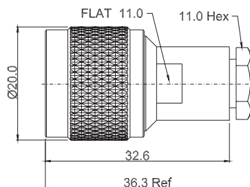
EN-2902 N MALE CLAMP STRAIGHT FOR CABLE - RG 174/U - RG 316/U
