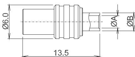
EMX-3802 MCX JACK SOLDER FOR CABLE - SEMI-RIGID - OD 2.5M - RG 316/U
