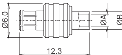
EMX-3903 MCX MALE SOLDER FOR CABLE - SEMI-RIGID - OD 2.5M - RG 3.6MM
