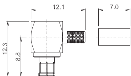
EMX-3902 MCX MALE R/A CRIMP FOR CABLE - RG 174/U - RG 316/U - MINI Rg62
