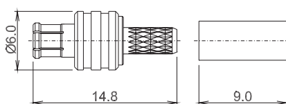
EMX-3901 MCX MALE STRAIGHT CRIMP FOR CABLE - RG 174/U - RG 316/U - MINI Rg62
