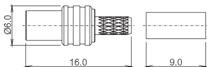
EMX-3801 MCX JACK STRAIGHT CRIMP FOR CABLE - RG 174A/U - RG 179B/U - RG 316/U
