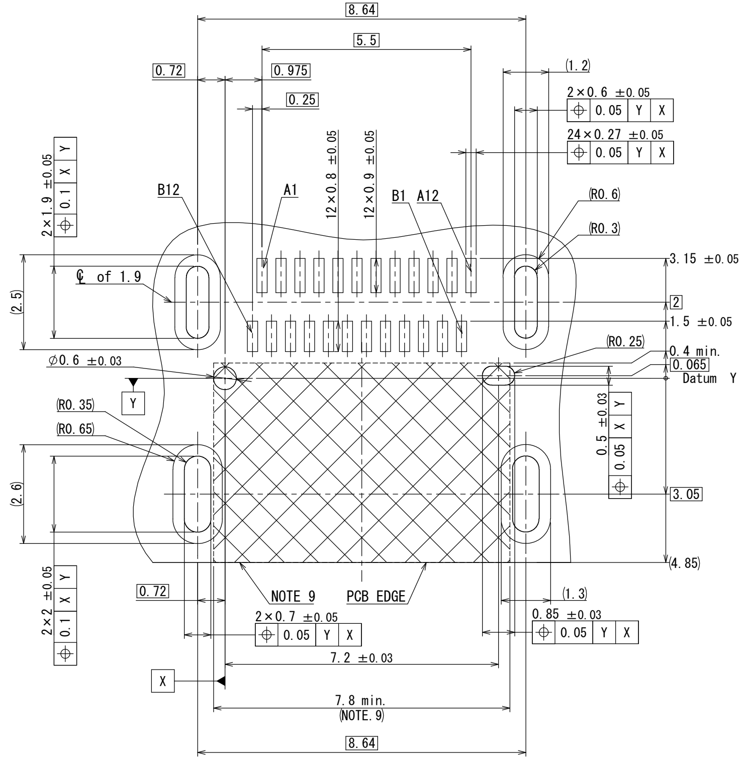
SURFACE VIEW FROM CONNECTOR MOUNTING SIDE APPLICABLE P.C.B DIMENSION (REF.) 適合基板寸法 (参考)
