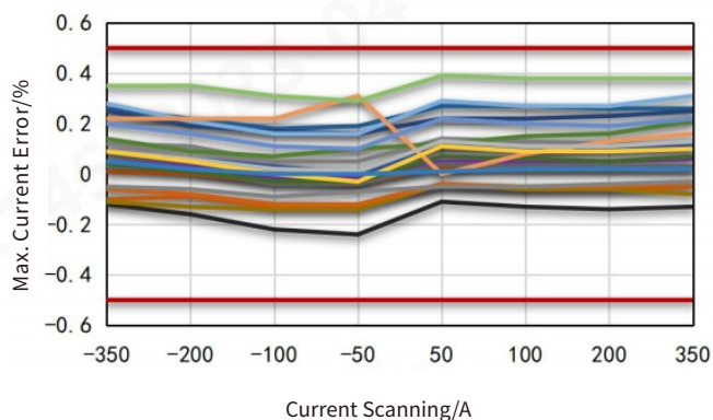
Figure 5-23 +85°C High-Current Test Accuracy@Max. Current Error
