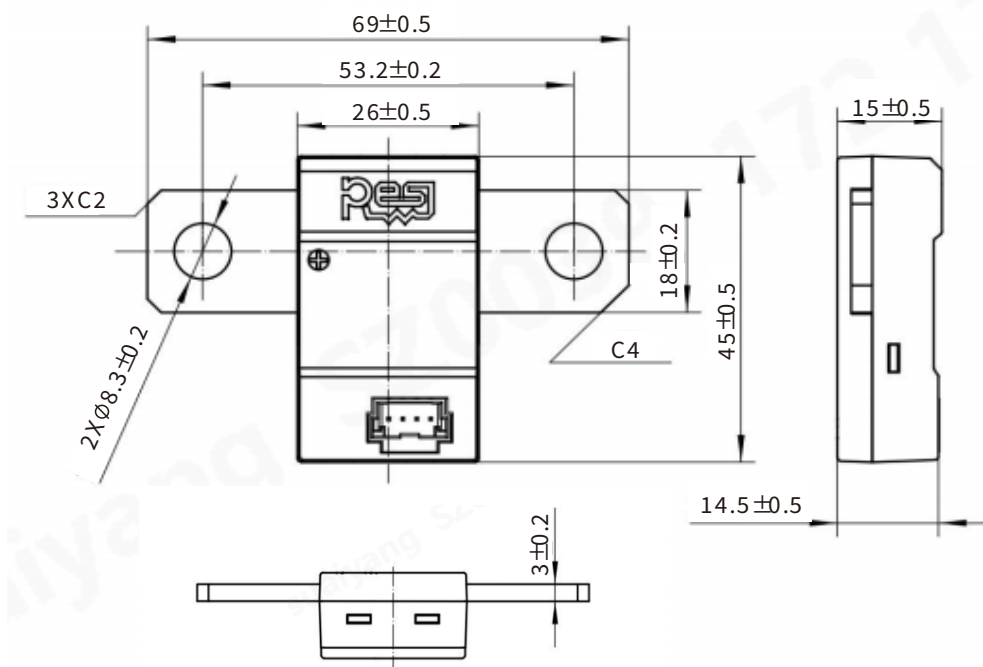
Figure 8.1 Structure Diagram
